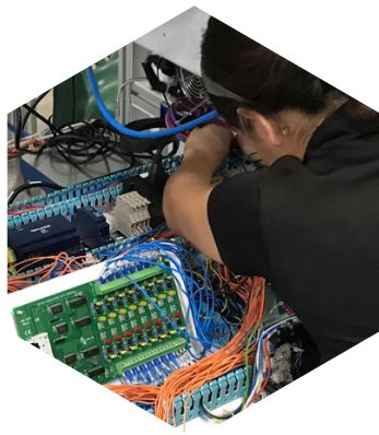
SOFTWARE ENGINEERING
